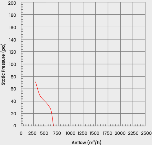
Airflow Curve:
