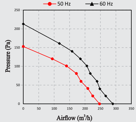
Airflow Curve:
