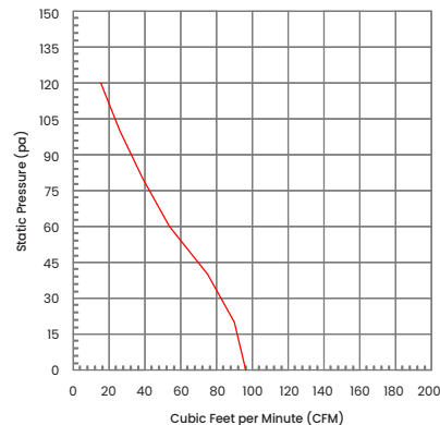
Airflow Curve:
